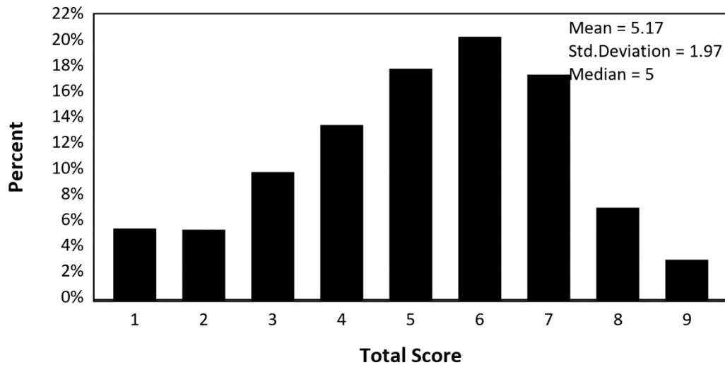
Frequency Table – PREview Scores
